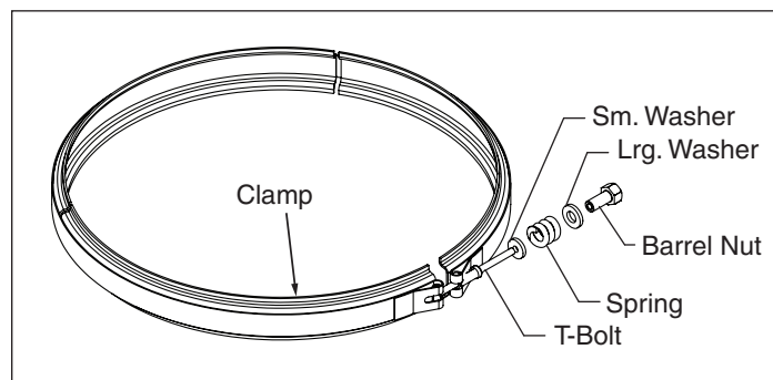
Figure 2: Clamp Assembly
